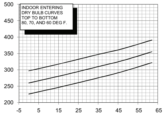
TEM6A0D48H41 Heating @ 1450 SCFM
